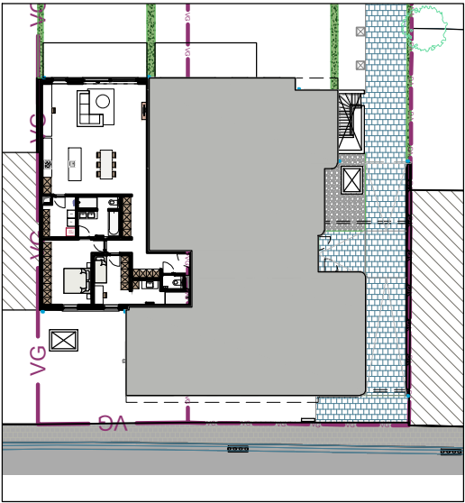
Verdiepingsplan +00
